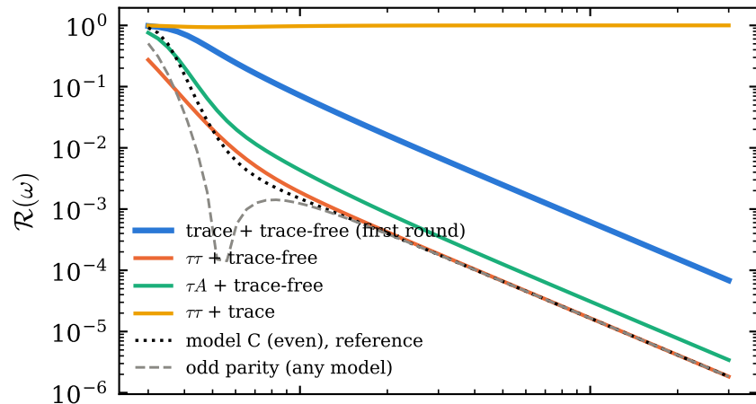
frozen domain wall (model A), \ell = 2 , R = 3M
