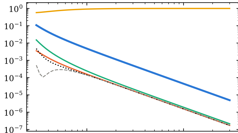
frozen domain wall (model A), \ell = 2 , R = 6M
